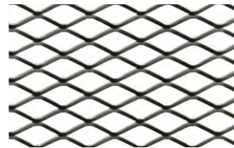
Model: ABE-P008 Mesh shape: rhomboidal Mesh size: 20mmx10mmx2mm
