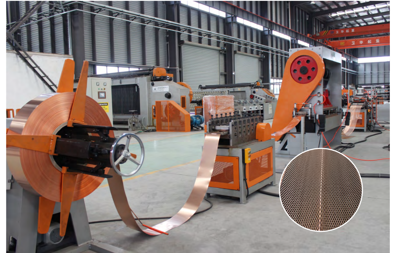
铜极网生产线 / Copper Battery Mesh Expanding line
